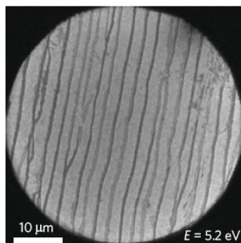
Fig. 1: LEEM image of graphene grown on SiC in an atmosphere of Ar
